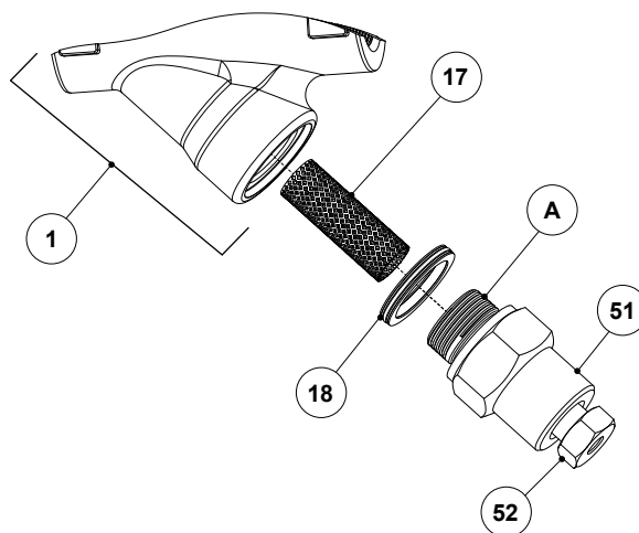
Fig. 4 – BDV blowdown valve
