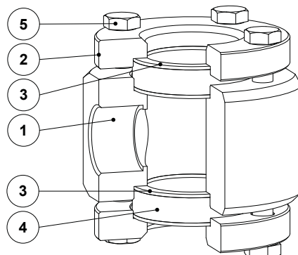
Fig. 4 - DW40 (1 1/4" to 2" – DN 32 to 50)
