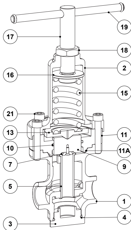
1" – DN 25
