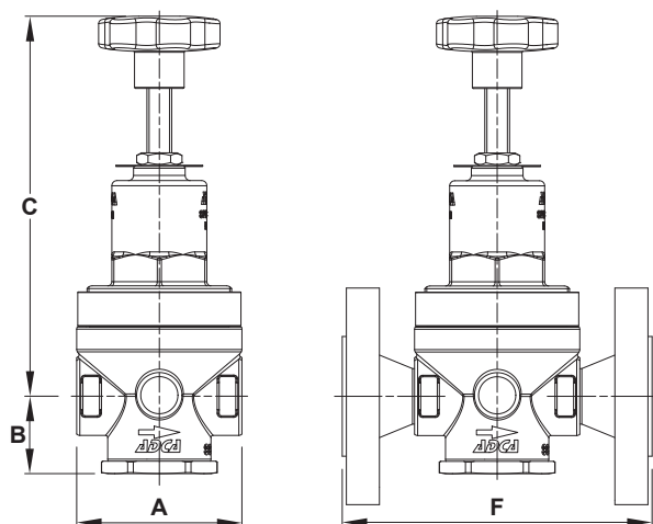
1/2" and 3/4" – DN 15 and DN 20
