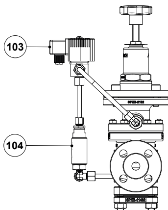
Valve with solenoid valve for remote closure
