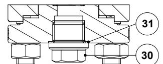
Detail C Optional drain connection
