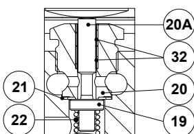
Detail A Pilot valve
