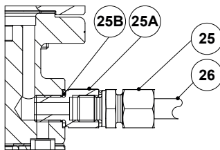
External sensing
