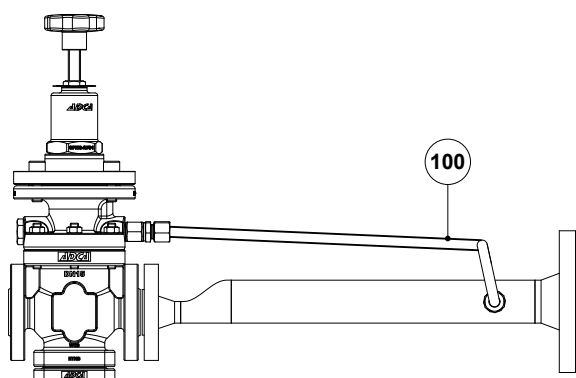
Standard valve
