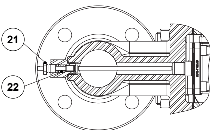
Optional steam lock release (SLR)
