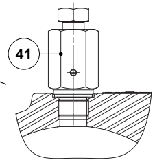
Optional hand vent valve (HVV)
