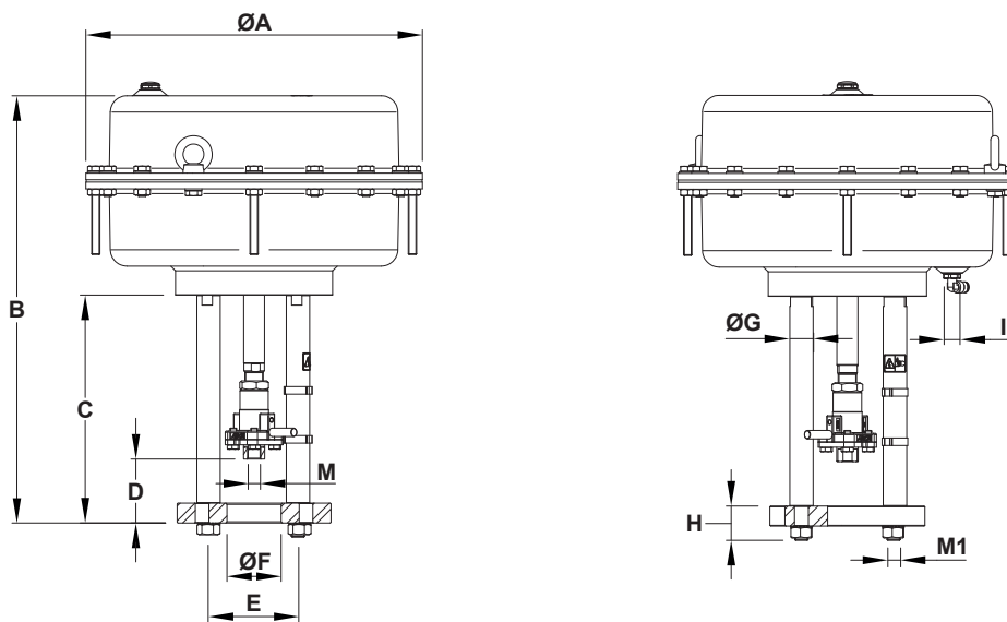
DIMENSIONS (mm)
