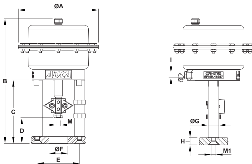
DIMENSIONS (mm)
