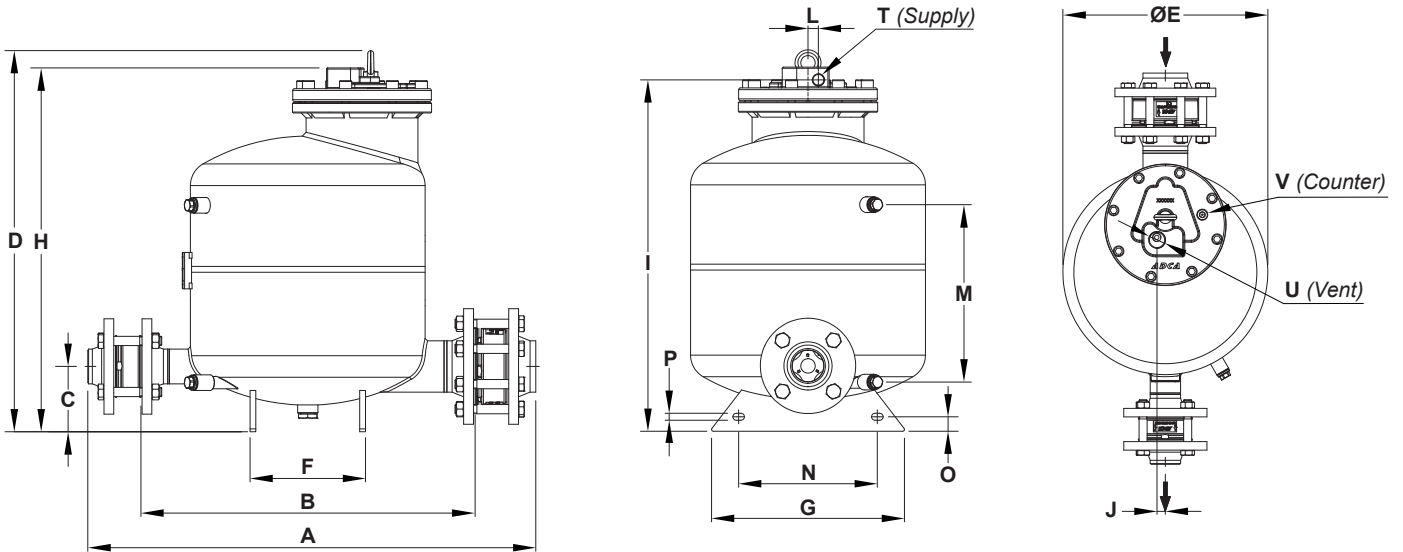
DIMENSIONS (mm)
