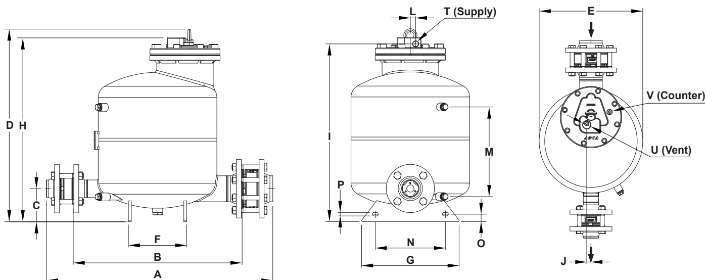
DIMENSIONS (mm)
