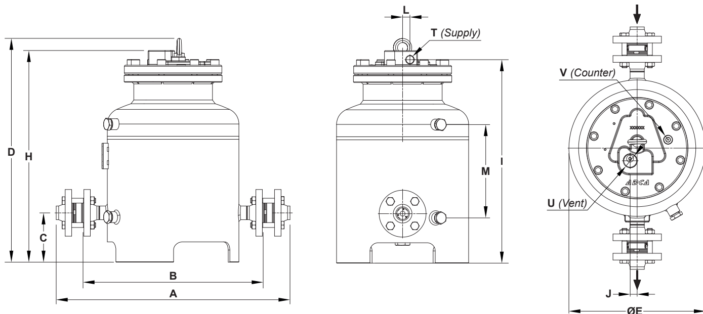
DIMENSIONS (mm)
