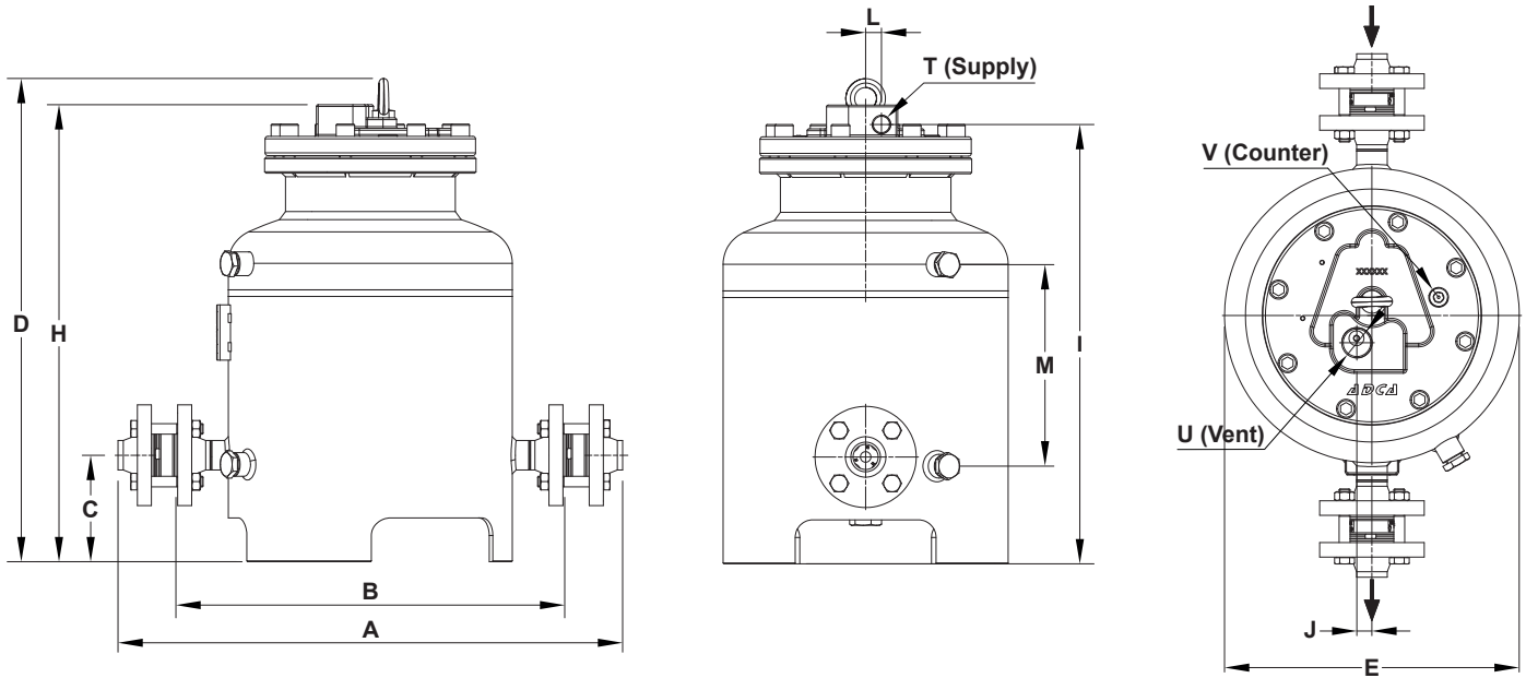
DIMENSIONS (mm)
