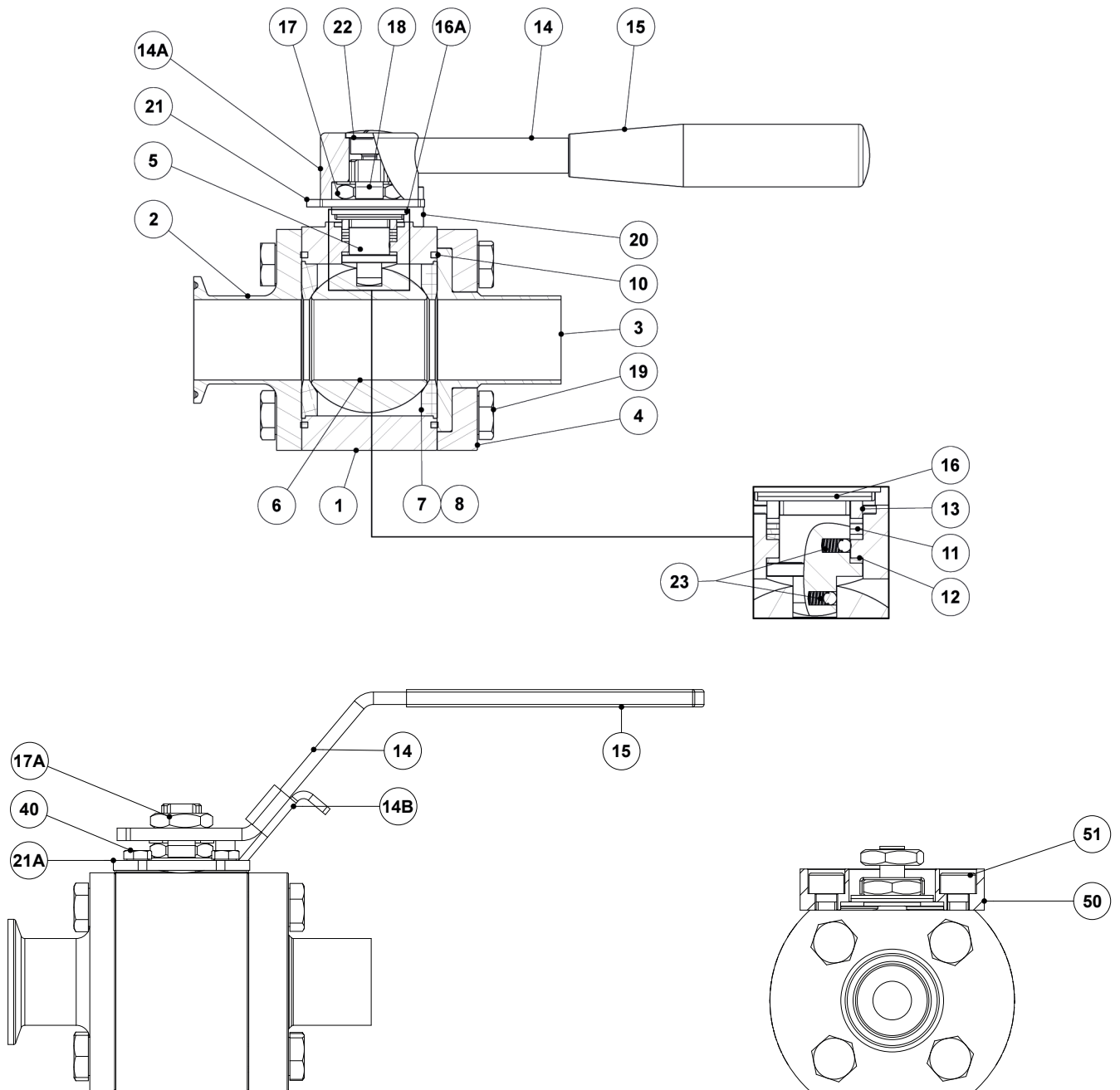
Optional flat lever with locking system
