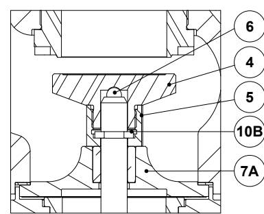
Detail A (DN 80 and DN 100)
