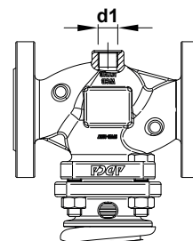
Optional sensing line connection on body (DN 15 to DN 25)
