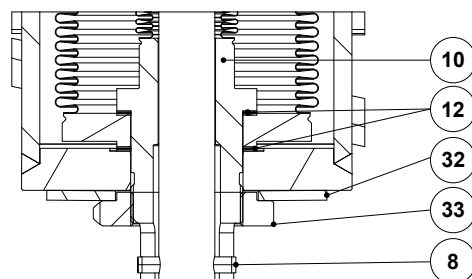
Detail C (DN 125 and DN 150)
