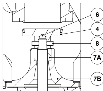
Detail A (2" and 21/2")
