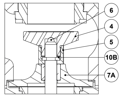
Detail A (3" and 4")
