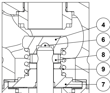
Detail A (1/2" to 11/2")
