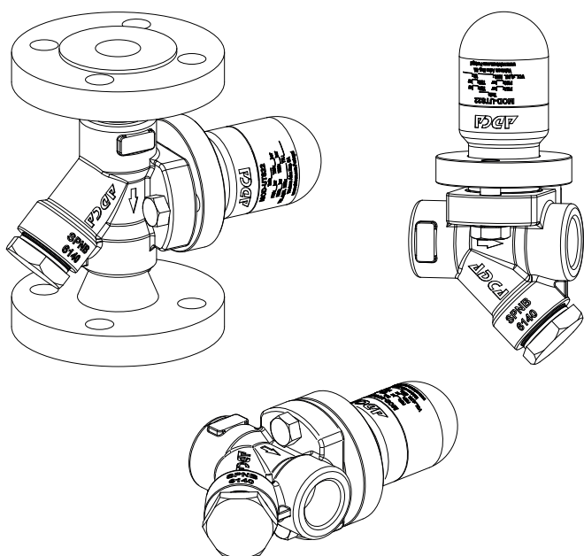
UTS22 steam trap connected to a UCX41 universal pipeline connector
