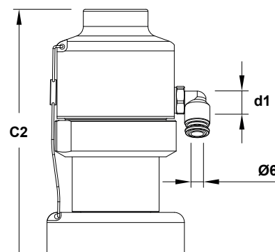
Optional pneumatic lifting device
