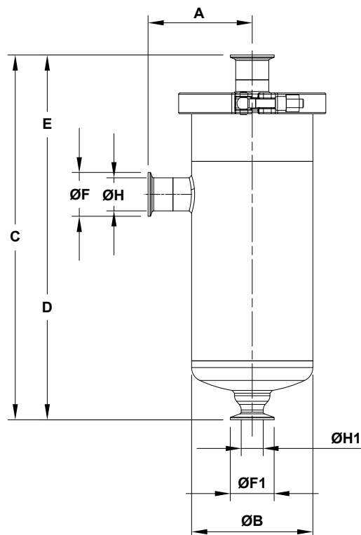
DIMENSIONS (mm)
