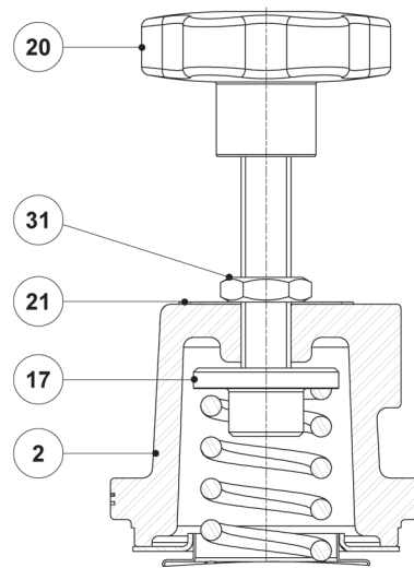
Optional rising adjustment knob
