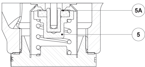
Soft sealing
