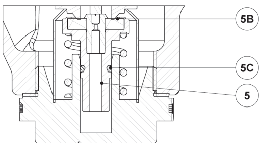
Balanced soft sealing (PRW)
