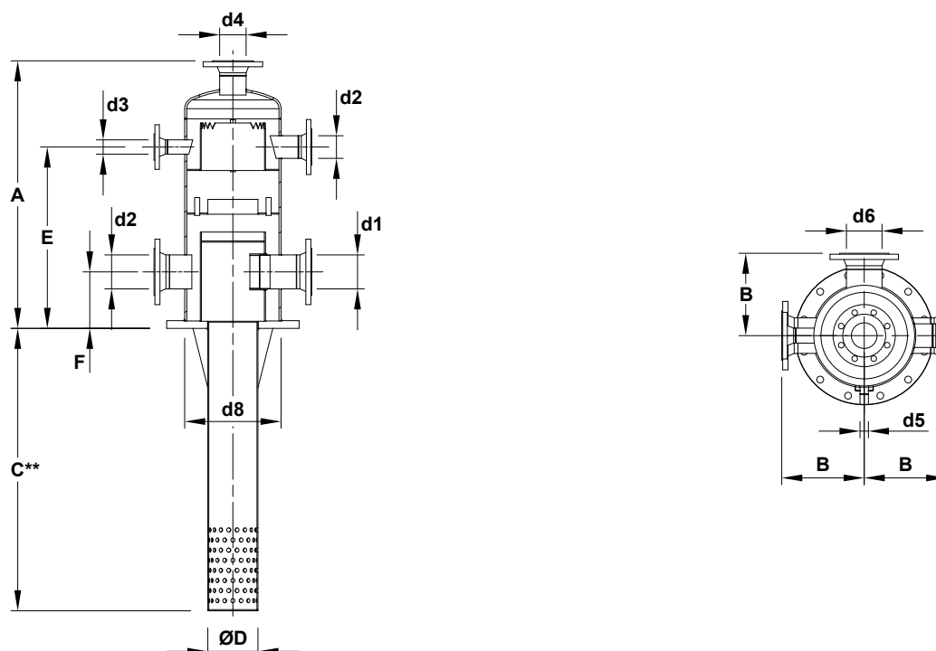
DIMENSIONS (mm)
