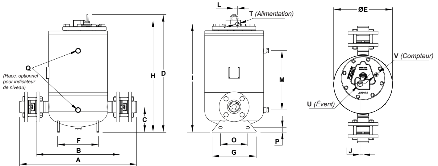
DIMENSIONS (mm)
