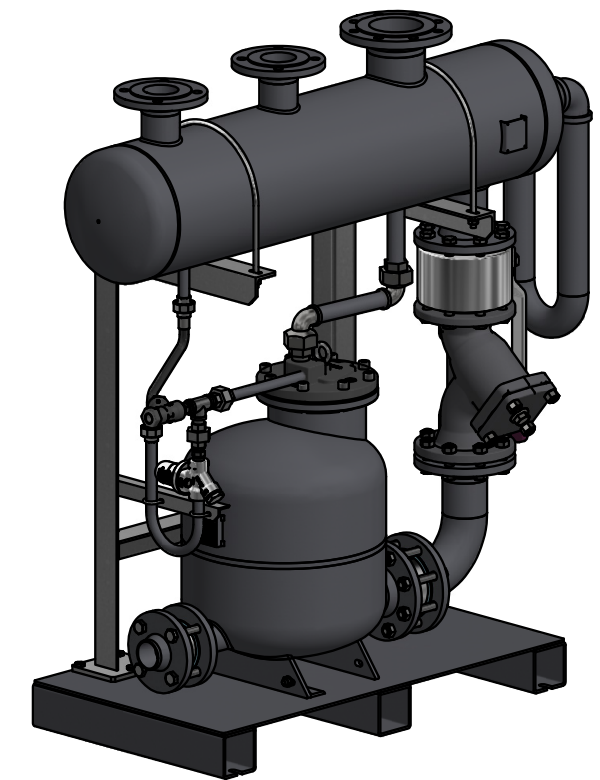
DN80x50
