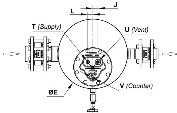
DIMENSIONS (mm)
