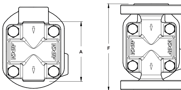
Horizontal Installation (R-L)
